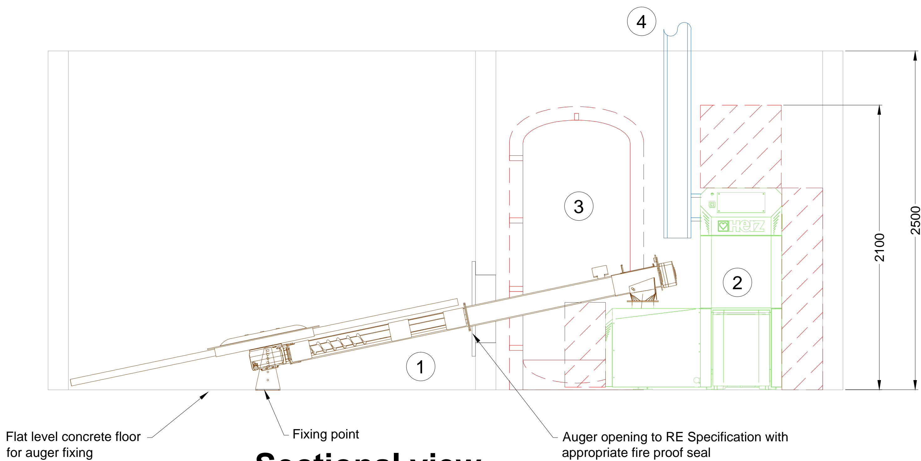
Sectional view
