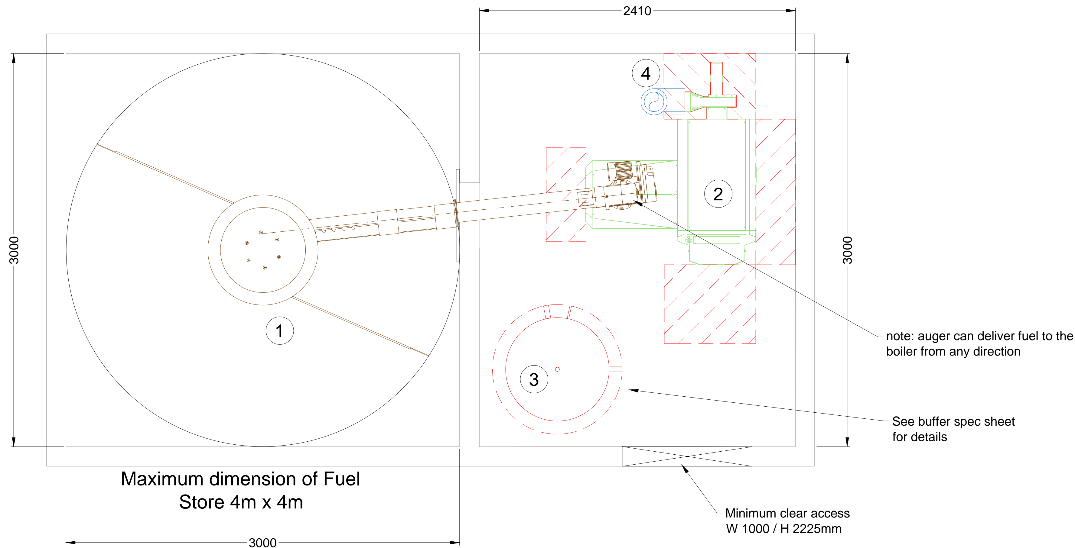
Plan View
