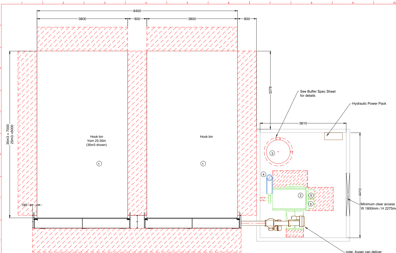
Plan View
