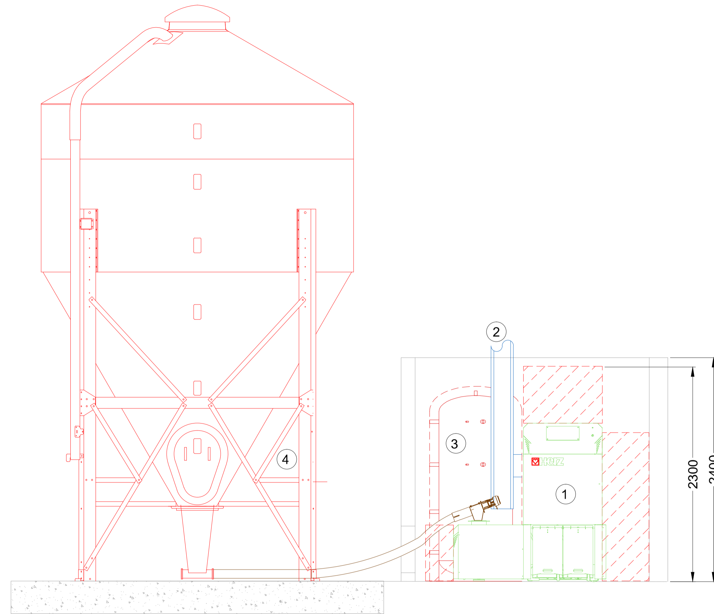
Sectional View
