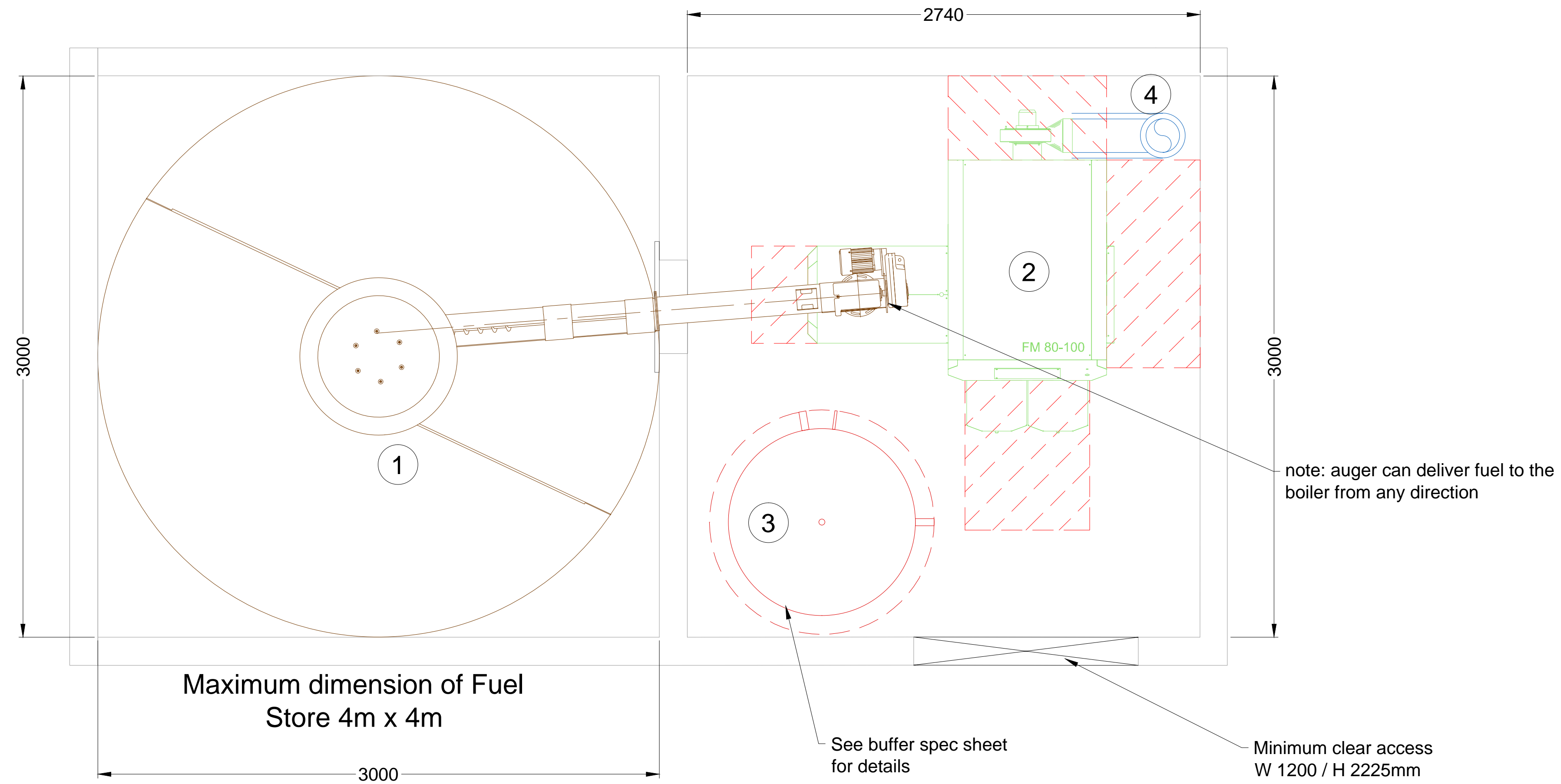
Plan View
