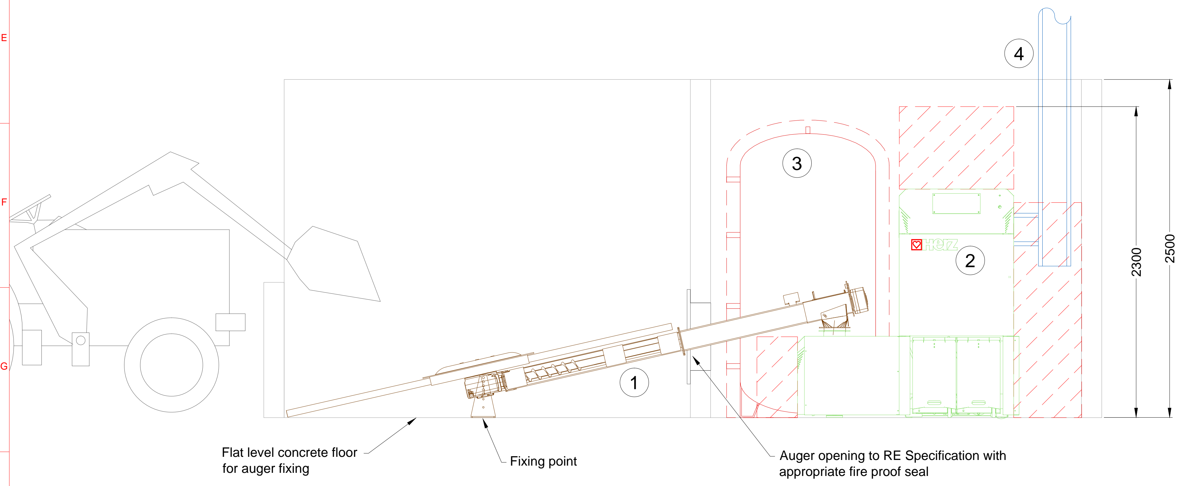
Sectional View
