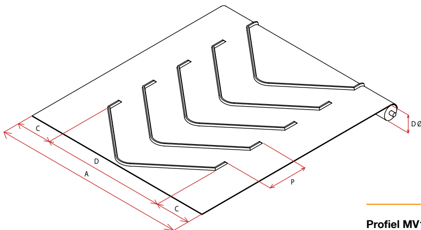
Profiel MV1400/22
